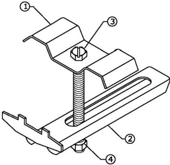
ASSEMBLED VIEW
